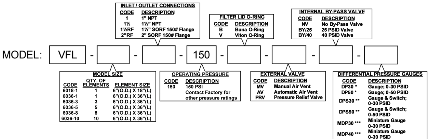
Cartridge Style Vessel (Model VFL-6036-1-2-150)
